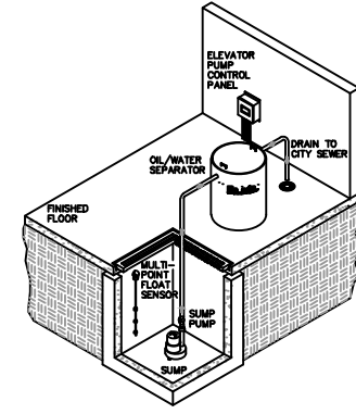
3 ELEVATOR SUMP SYSTEM SCHEDULE NOT TO SCALE
