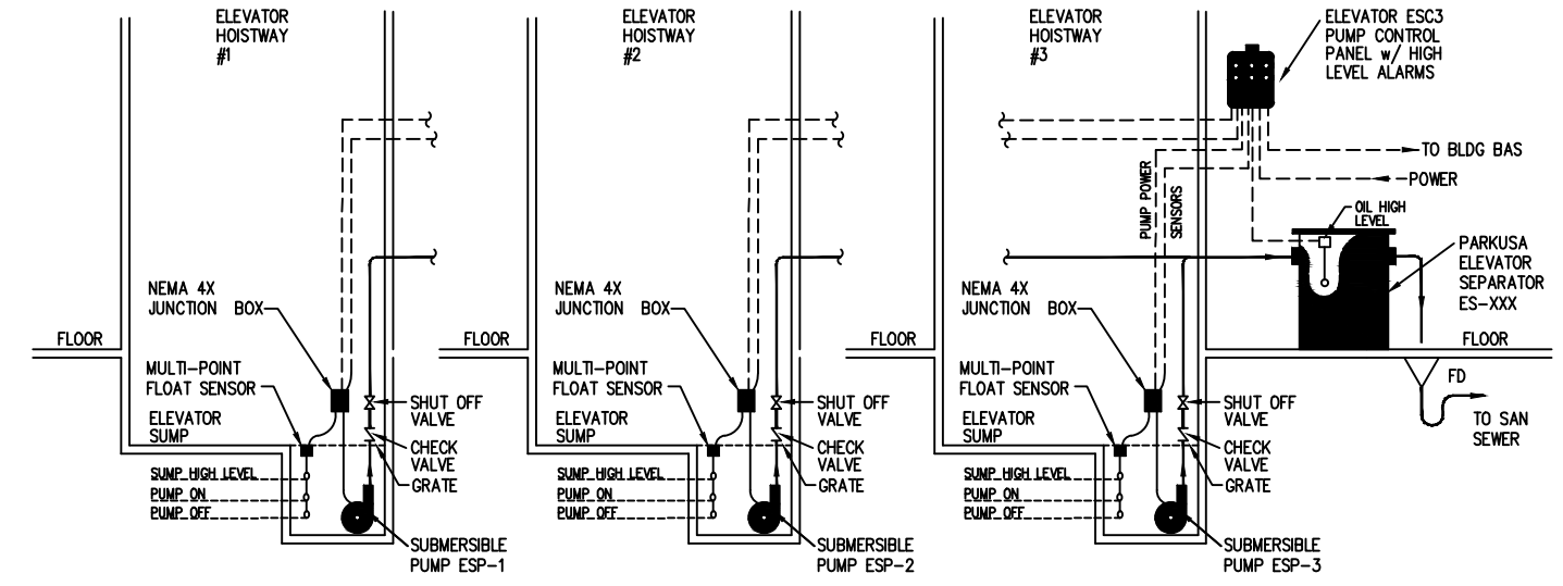
1 ELEVATOR SUMP DETAIL NOT TO SCALE (BELOW GRADE SEPARATOR)
