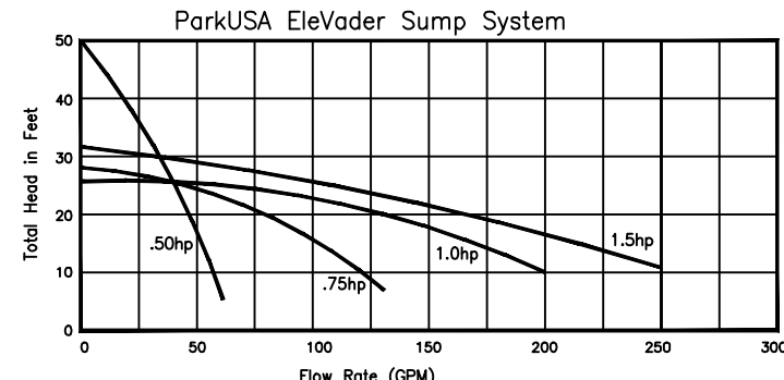
4 PUMP CURVE NOT TO SCALE
